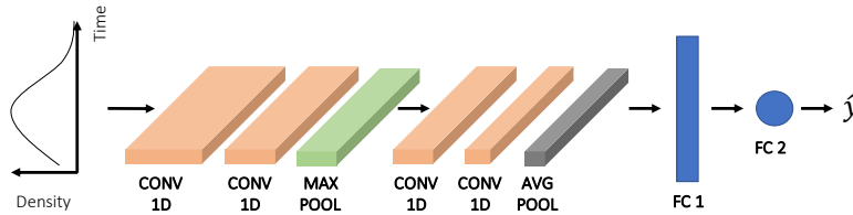
Figure 7: Schematic diagram representing the 1D convolutional architecture used for model 4 (modified from LLC 2021). It is composed of two CONV 1D + POOL blocks followed two FC layers, for a total of 49,511 trainable parameters. All CONV 1D layers in the first block are identical and composed of 30 filters of size 10. The MAXPOOL layer uses a window and stride of 3. The last two CONV 1D layers are composed of 50 filters of size 10. The average pool layer has a window length and stride set to 2.
