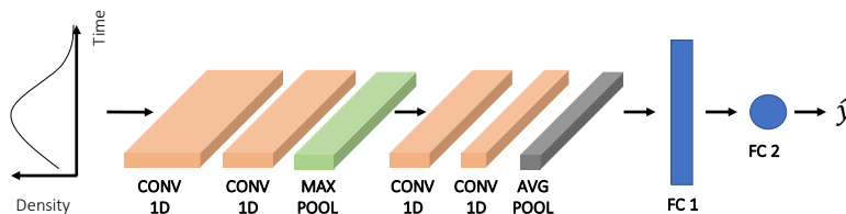
Figure 1: Schematic of the 1D convolutional architecture (modified from LLC 2021). It is composed of two CONV 1D + POOL blocks followed two FC layers, for a total of 49,511 trainable parameters.
